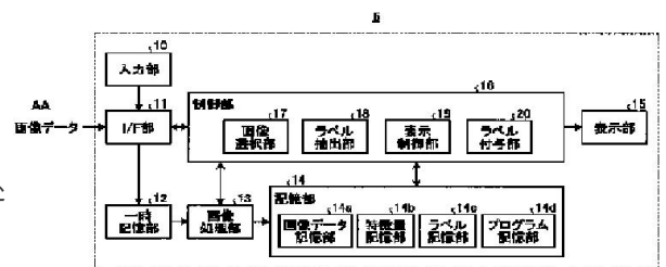
FIG. 2: AA: Image data 10: Input unit 11: I/F unit 12: Temporary storage unit 13: Image processing unit 14: Storage unit 14a: Image data storage unit 14b: Feature value storage unit 14c: Label storage unit 14d: Program storage unit 15: Display unit 16: Control unit 17: Image selection unit 18: Label extraction unit 19: Display control unit 20: Labelling unit
